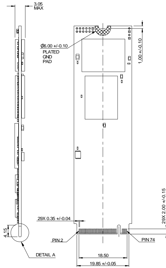
BOTTOM VIEW
