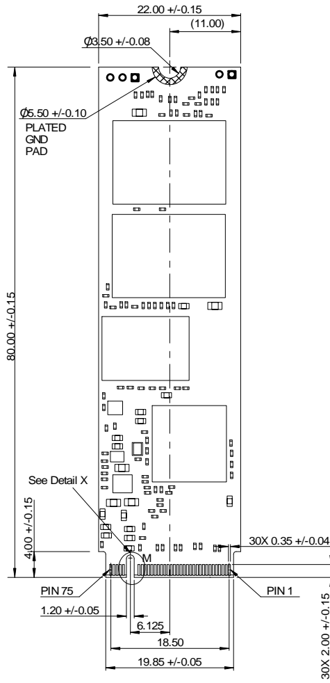
TOP VIEW
