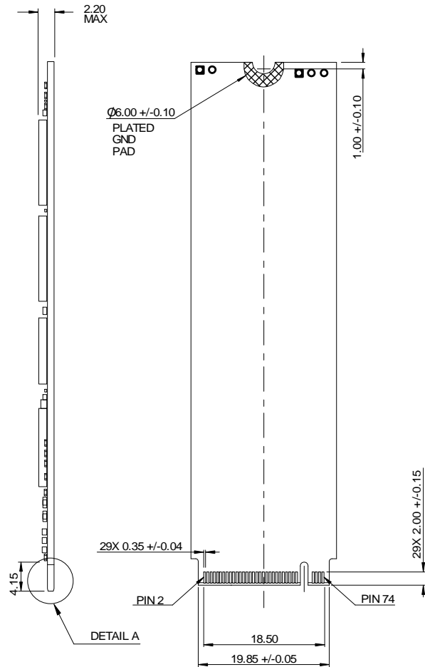
BOTTOM VIEW
